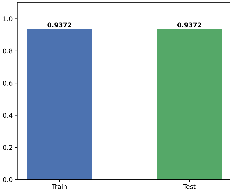
F1-Scores MPE
