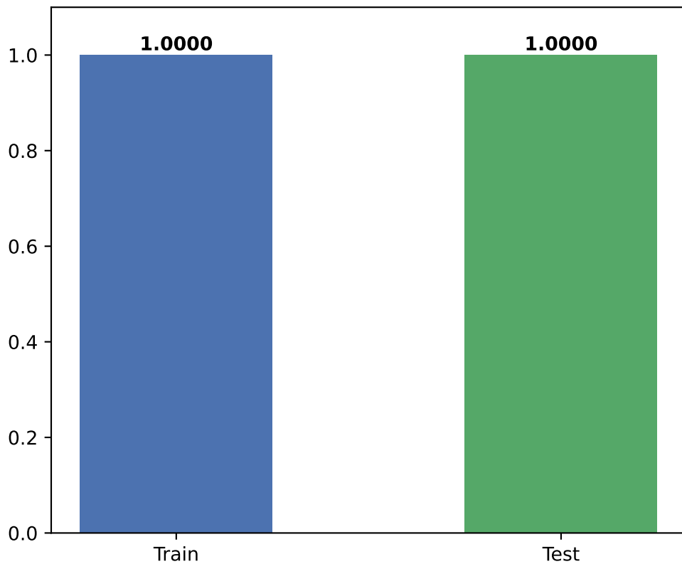
F1-Scores MPE
