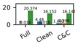
Meteor
