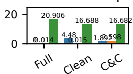
ReverseComp
