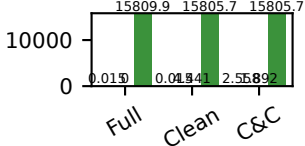
Chameleons
