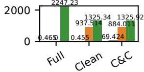
DeltaBlue
