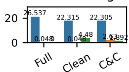
ThreadRing
