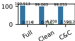
RegexDNA
