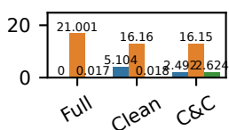
NBody
