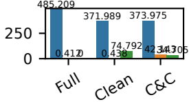
Compiler
