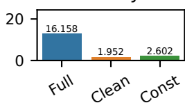
ReverseComp
