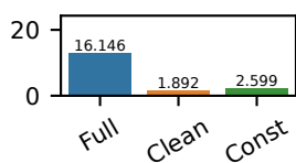
Meteor
