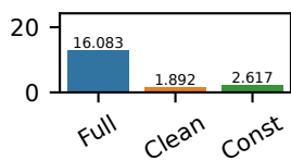
BinaryTrees
