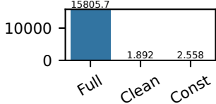
Chameleons
