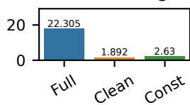
ThreadRing
