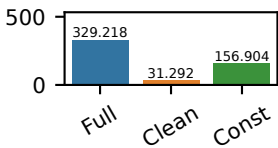
Richards
