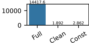
KNucleotide
