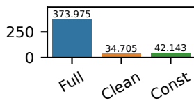
Compiler
