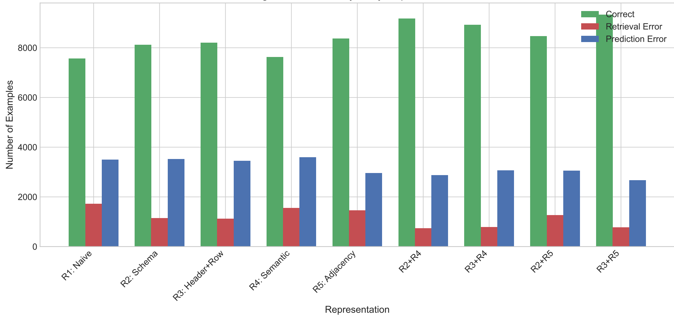
Figure 5: Error Analysis by Representation
