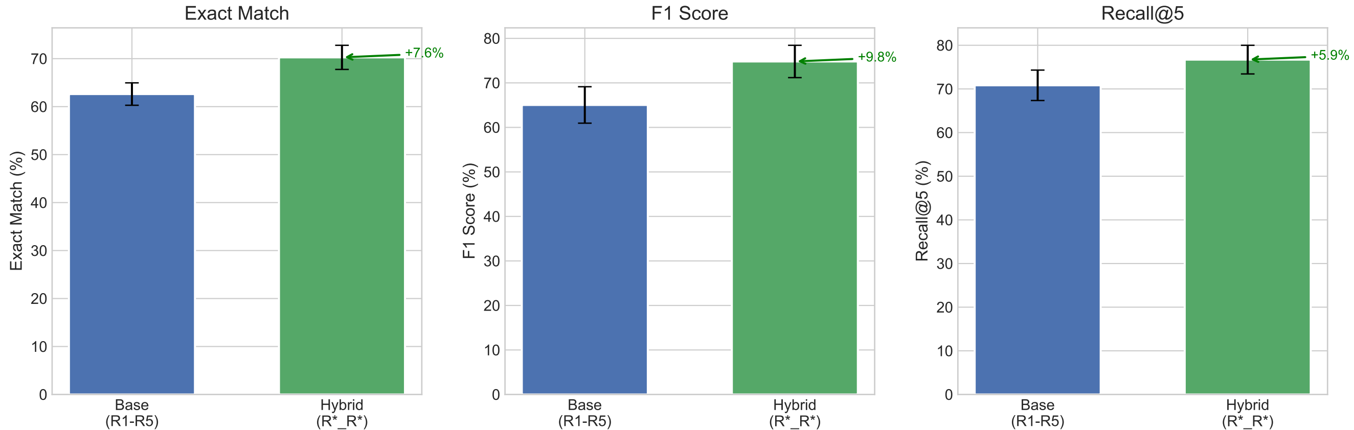
Figure 6: Base vs Hybrid Representation Performance
