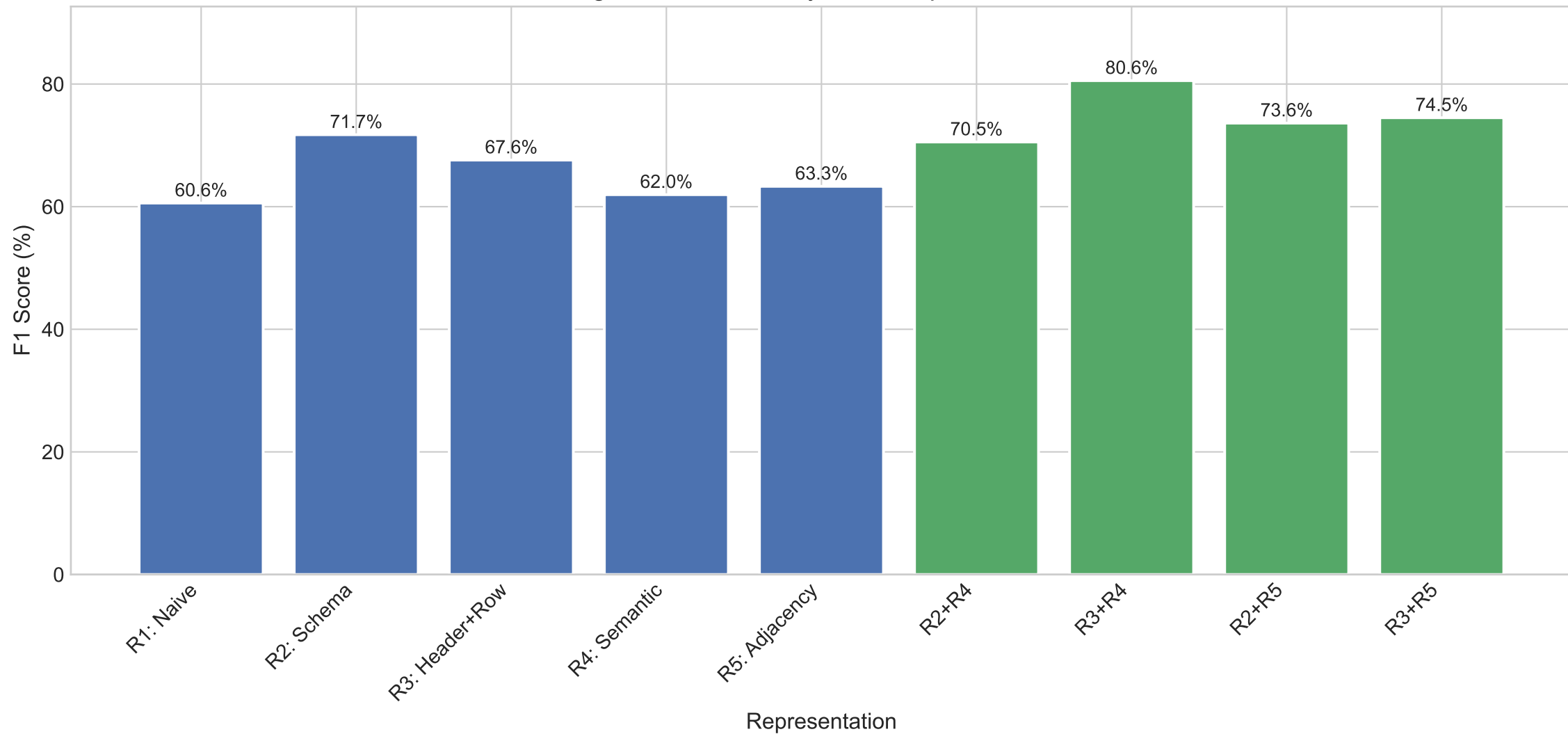
Figure 2: F1 Score by Table Representation
