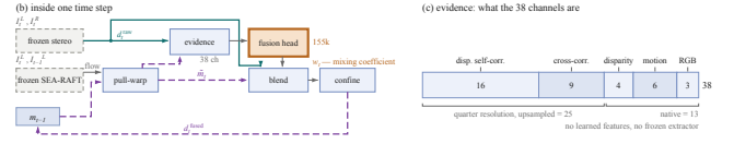
Fig. 1. (b) One time step; dashed grey is frozen, the single orange block is the only trained component and emits one scalar per pixel, w_t , rather than geometry. (c) The evidence space: none of the 38 channels carries ground truth, backbone identity or a future frame.
