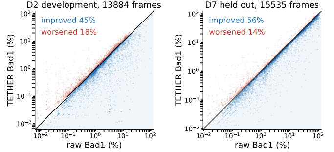
Fig. 2. Per-frame Bad1, raw against refined, for every scored frame of each split — five backbones, all sequences, no selection. Points below the diagonal are improved. The worsened band hugs the diagonal while the improved mass extends far from it: the frame-level count-versus-magnitude asymmetry behind B^+/H^+ . On held-out D7, 56% of the 15,535 frames improve against 14% worsened; on development D2 the split is 45% against 18%, so the frame-level margin is wider on the split that took no part in any choice.
