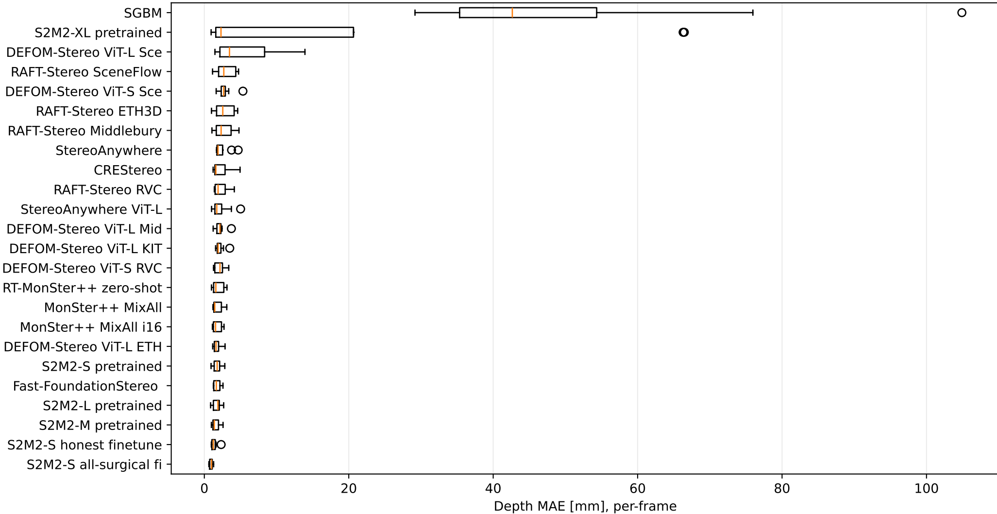
SERV-CT holdout per-frame depth MAE distribution
