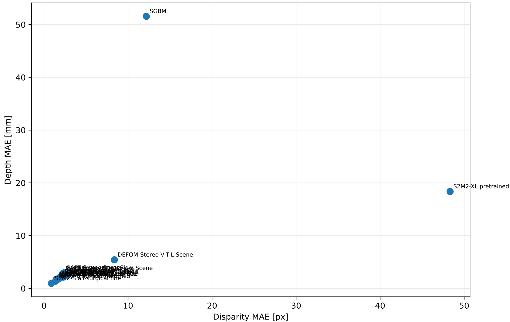
Accuracy Pareto proxy: depth MAE vs disparity MAE (runtime unavailable)
