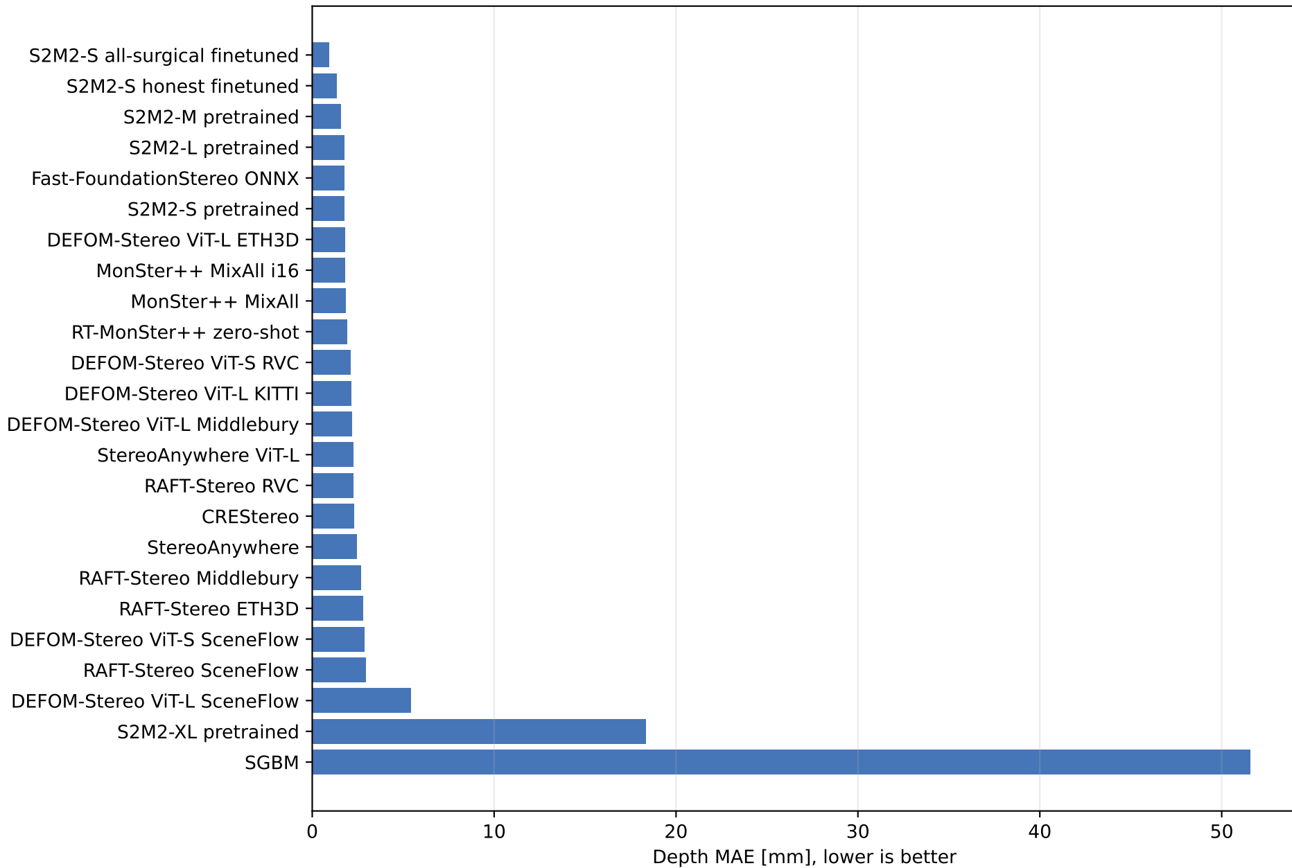
SERV-CT holdout method ranking
