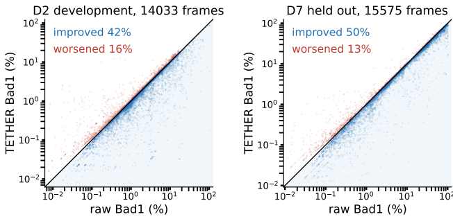
Fig. 2. Per-frame Bad1, raw against refined, for every scored frame of each split — five backbones, all sequences, no selection. Points below the diagonal are improved. On D7 half improve against 13% worsened, and the worsened band hugs the diagonal while the improved mass extends far from it: the frame-level form of the count-versus-magnitude asymmetry behind B^+/H^+ . Disparity maps are not shown — the intervention is sub-pixel on disparities of about 8 px.
