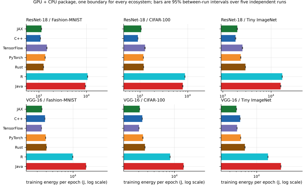
Fig. 2: Training energy per epoch, accelerator plus CPU package, with 95% Student- t intervals over 5 independent runs. Note the logarithmic axis: the intervals are narrow enough to be hard to see at this scale.
