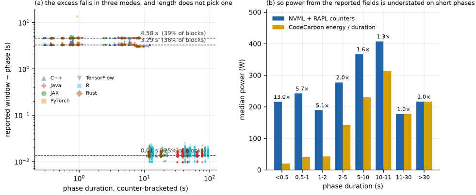
Fig. 5: (a) The duration reported alongside each energy figure is not the interval the energy was accumulated over: the excess falls into 3 discrete modes, one per outstanding network lookup in stop() , with a threshold near 11 s. (b) Power obtained by dividing reported energy by reported duration is consequently understated for short phases and exact above 11 s. Both instruments are compared on the terms both measure.
