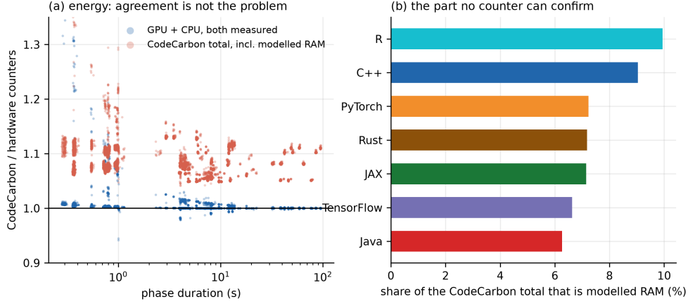
Fig. 6: (a) Ratio of CodeCarbon to hardware counters, per block, against phase duration. The measured part agrees; the total does not, by exactly the modelled RAM term. (b) The share of each ecosystem’s reported total that is modelled RAM.
