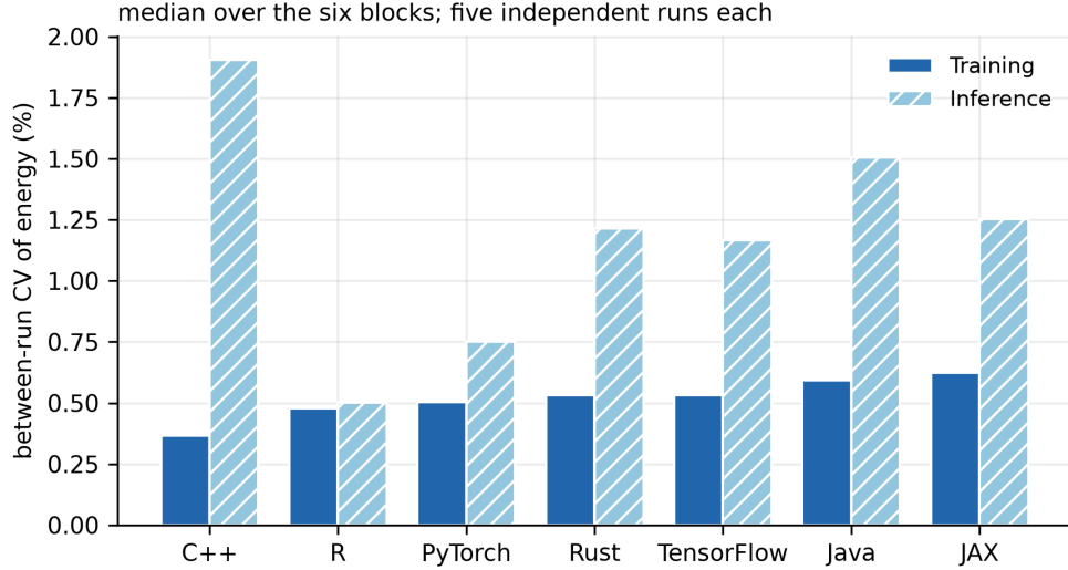
Fig. 1: Between-run coefficient of variation of energy, median over the six (model, dataset) cells, from 5 independent runs per configuration.
