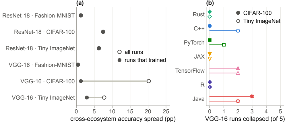
Fig. D.1: The superseded first campaign, from that campaign’s own records. (a) Cross-ecosystem accuracy spread per cell, over all runs (hollow) and over only the runs that trained (filled); the gap on VGG-16 is the collapsed runs. (b) VGG-16 runs that collapsed to chance, out of 5 per cell, on CIFAR-100 (filled) and Tiny ImageNet (hollow). The same figure for the campaign reported here is not drawn: with 0 collapses its panel (a) plots one set of runs against itself and its panel (b) is empty in every cell.
