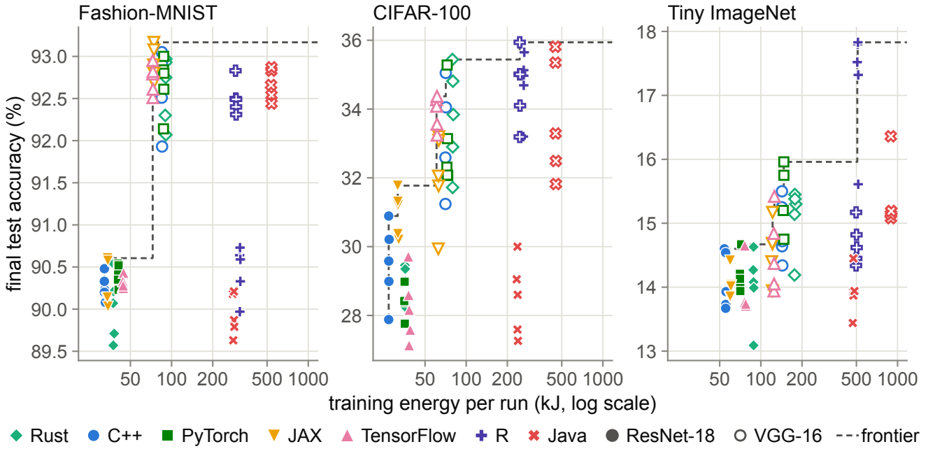
Figure 3: Energy spent against accuracy reached, one point per run (filled: ResNet-18, hollow: VGG-16; one logarithmic energy axis). Dashed: the empirical frontier, left of which no configuration reaches the same accuracy.
