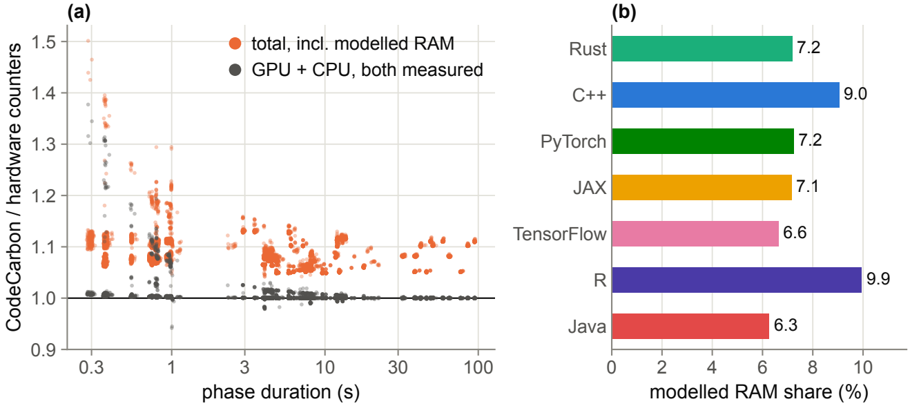
Figure 5: (a) CodeCarbon over the counters, per block, against phase duration: the GPU and CPU terms both measure (grey) agree; the total (orange) exceeds them by the modelled RAM term. (b) Mean modelled-RAM share of each ecosystem’s reported total.
