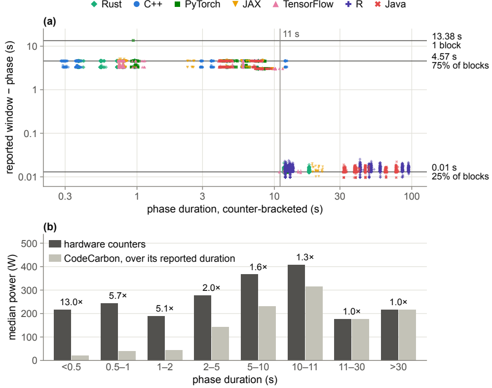
Fig. 4: (a) Per block, the reported duration minus the counter-bracketed phase, against the phase: 3 modes (horizontal lines, with median and share of blocks) and the threshold near 11 s (vertical line). (b) Median power per phase-length bin from the counters and from reported energy over reported duration, on the terms both measure, labelled with the median factor by which the second understates the first (Online Resource 1, Table E.3).
