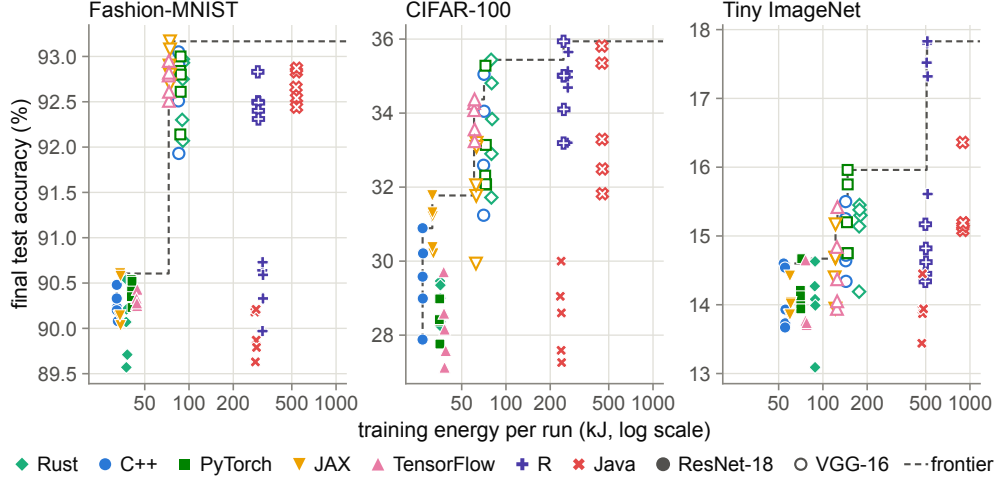
Fig. 3: Energy spent against accuracy reached, one point per run (filled: ResNet-18, hollow: VGG-16; one logarithmic energy axis). Dashed: the empirical frontier, left of which no configuration reaches the same accuracy.
