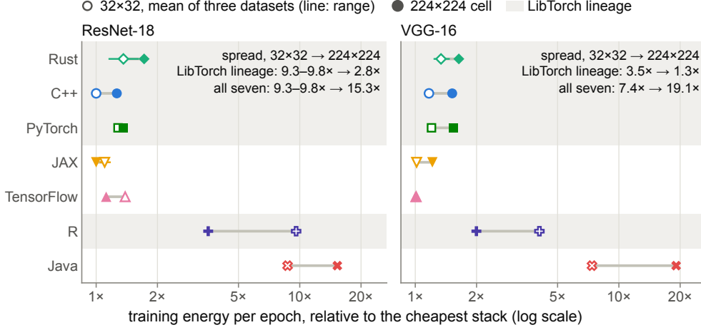
Fig. 6: Per-epoch training energy (mean over runs of each run’s per-epoch counter mean, as in the spread rows of Table 9) as a multiple of the cheapest stack in the same regime: 32 \times 32 (hollow; mean of the three datasets, each normalised to its own cheapest, range as a coloured line) and the 224 \times 224 cell (filled). On the log axis distance is spread. Shaded rows: the LibTorch lineage.
