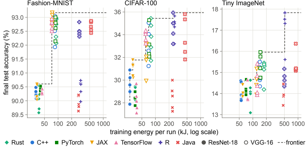
Fig. 3: Energy spent against accuracy reached, one point per run; filled markers are ResNet-18 runs and hollow markers VGG-16 runs. The energy axis is logarithmic and the same in all three panels. The dashed line is the empirical frontier: no configuration to its left reaches the same accuracy for less energy.
