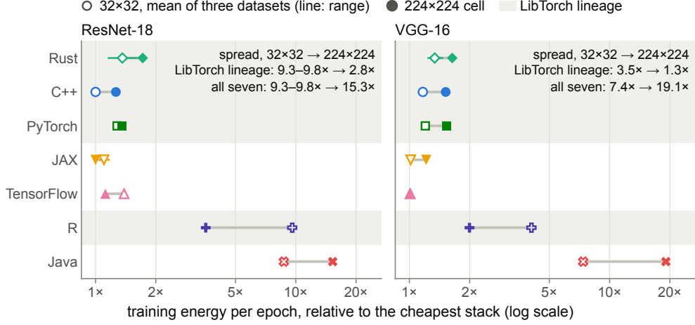
Fig. 7: Per-epoch training energy of each stack as a multiple of the cheapest of the seven in the same regime: at 32 \times 32 (hollow; the mean over Fashion-MNIST, CIFAR-100 and Tiny ImageNet, each normalised to its own cheapest stack, with their range as a coloured line where it is wider than the marker) and in the saturation cell at 224 \times 224 , batch 32, on Imagenette (filled). A stack’s energy in a regime is the mean over its runs of the run’s mean per-epoch counter energy, the definition behind the spread rows of Table 16. On the logarithmic axis the distance between two stacks is the spread between them. Shaded rows are the LibTorch lineage. The cell changes resolution, batch size and dataset together.
