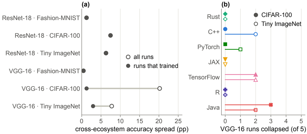
Fig. 4: The superseded first campaign, from that campaign’s own records. (a) Cross-ecosystem accuracy spread per cell, over all runs (hollow) and over only the runs that trained (filled); the gap on VGG-16 is the collapsed runs. (b) VGG-16 runs that collapsed to chance, out of 5 per cell, on CIFAR-100 (filled) and Tiny ImageNet (hollow). The same figure for the campaign reported here is not drawn: with 0 collapses its panel (a) plots one set of runs against itself and its panel (b) is empty in every cell.
