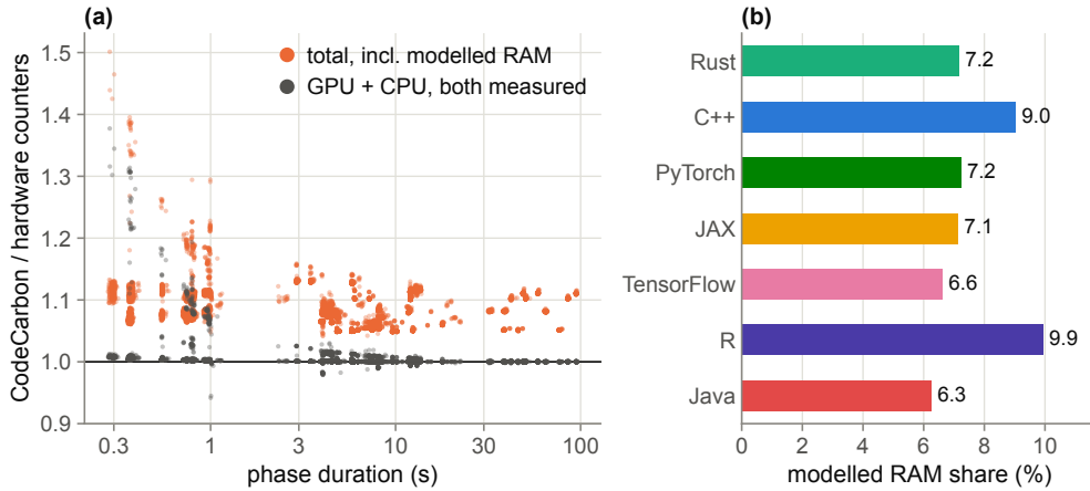
Fig. 6: (a) Ratio of CodeCarbon to hardware counters, per block, against phase duration, for the GPU and CPU terms both measure (grey) and for CodeCarbon’s total (orange). The measured part agrees; the total does not, by exactly the modelled RAM term. (b) The share of each ecosystem’s reported total that is modelled RAM, mean over its blocks.
