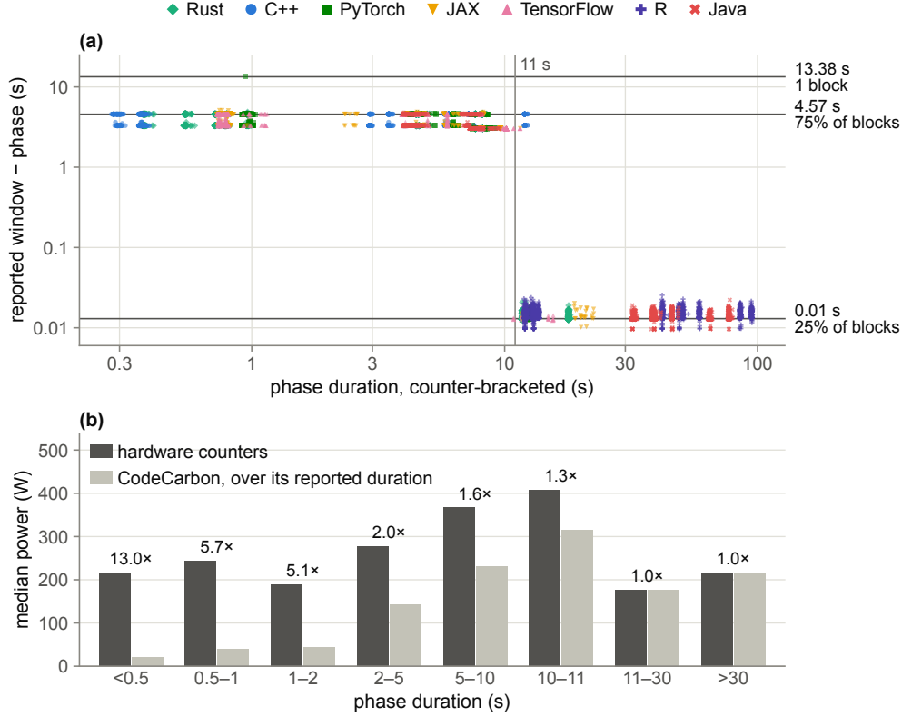
Fig. 5: (a) The duration reported alongside each energy figure is not the interval the energy was accumulated over. Each point is one block: the reported duration minus the counter-bracketed phase, against the phase. The excess falls into 3 discrete modes (horizontal lines, labelled with their median and share of blocks); the middle one holds both padded levels of Table 11, one and two network lookups outstanding in stop() , and the top one is a single block. The vertical line is the threshold near 11 s. (b) Median power per phase-duration bin, from the hardware counters and from reported energy divided by reported duration, on the bins of Table 13; the labels are the median factor by which the second understates the first. Power from the reported fields is understated for short phases and exact above 11 s. Both instruments are compared on the terms both measure.
