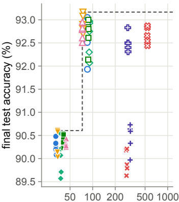
Fashion-MNIST
