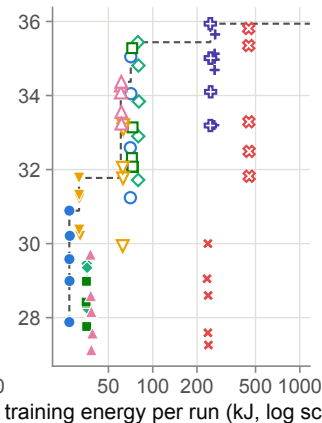
CIFAR-100
