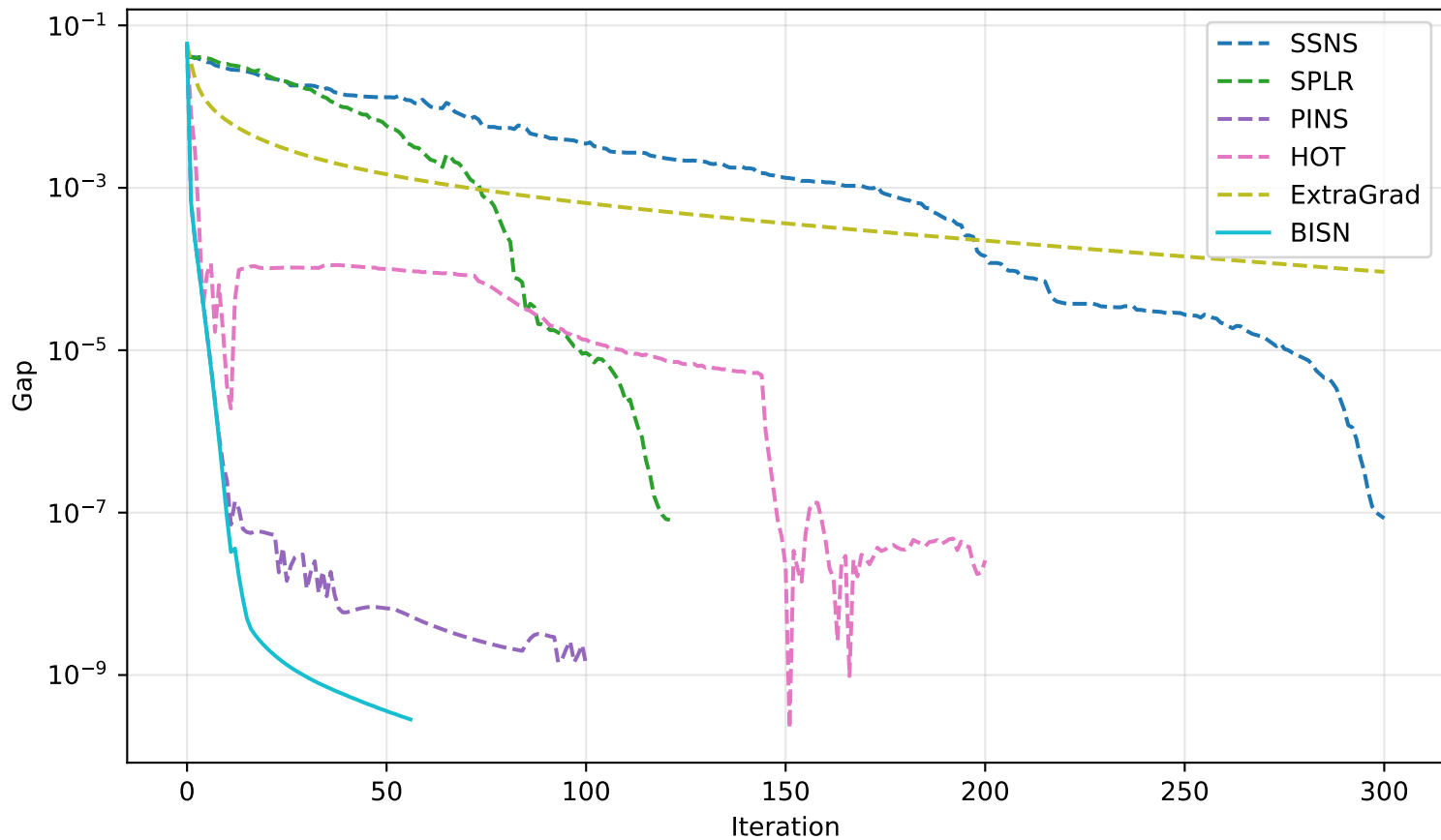
MNIST (ID1=3, ID2=12580)
