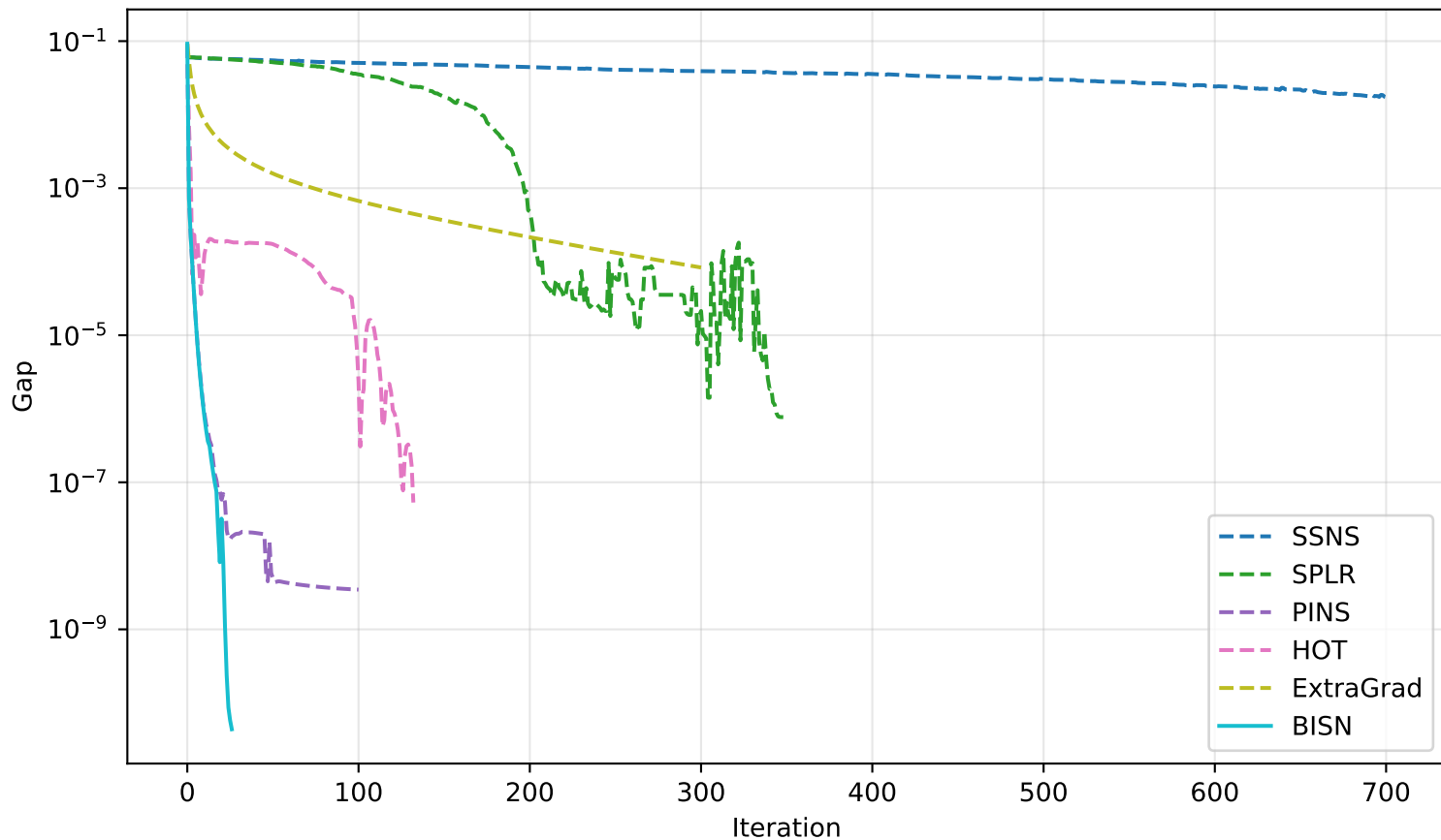
FashionMNIST (ID1=2, ID2=54698)
