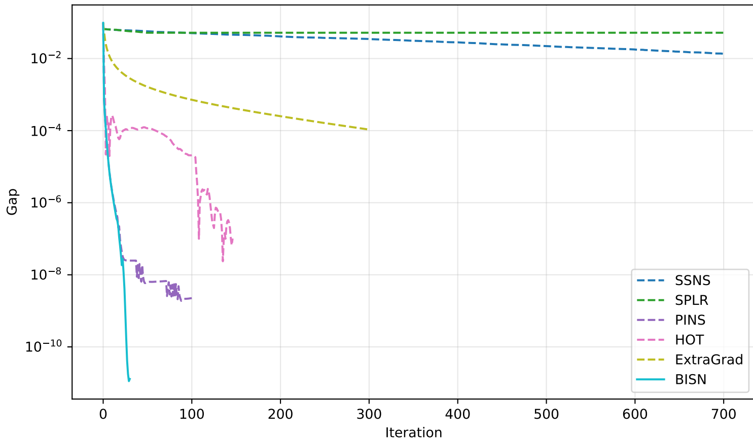
FashionMNIST (ID1=0, ID2=1)
