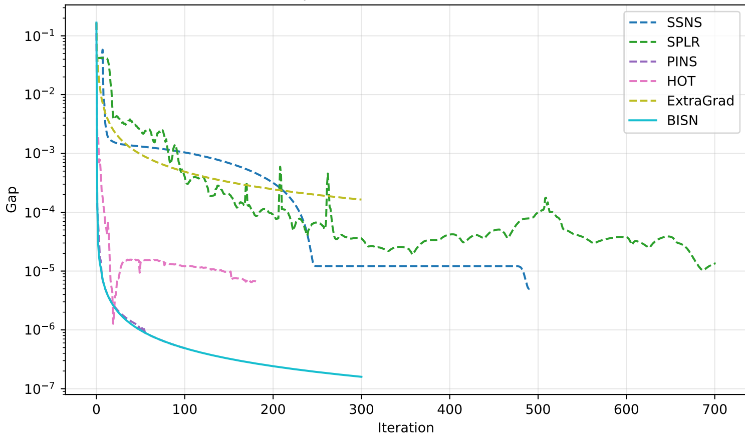
Square ( m=10000 , n=10000 )
