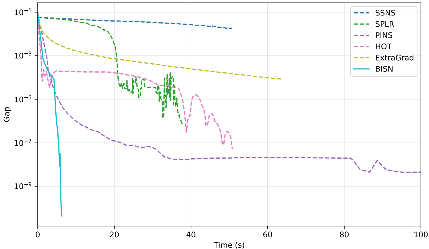
FashionMNIST (ID1=2, ID2=54698)
