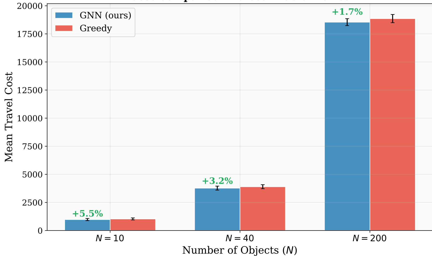
Cost Comparison Across Problem Sizes
