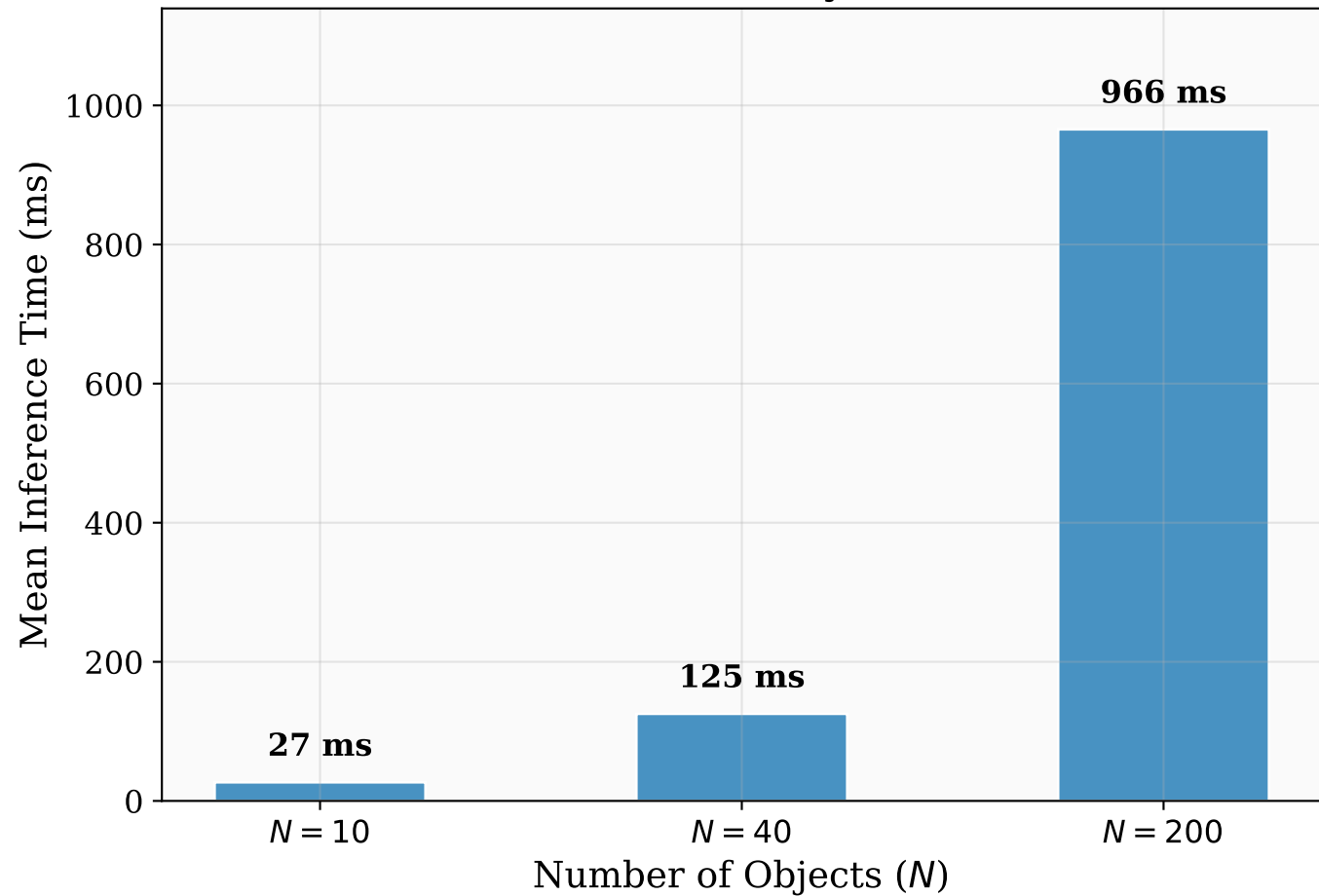
GNN Inference Time by Problem Size
