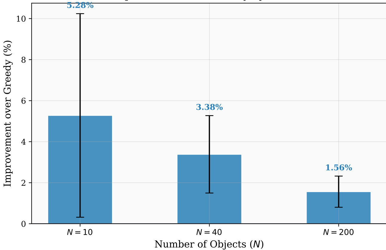
GNN Improvement over Greedy by Problem Size
