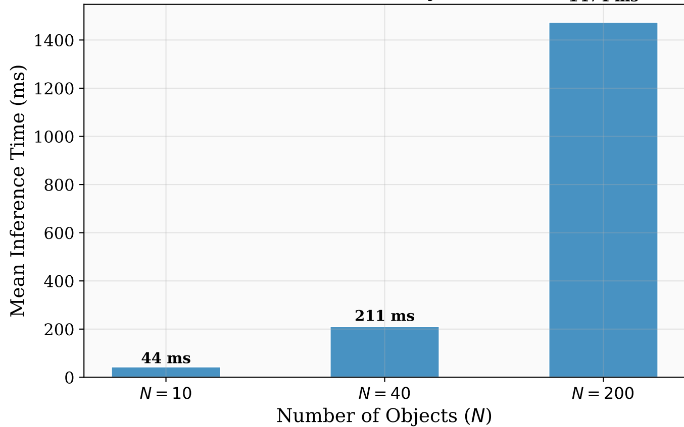
GNN Inference Time by Problem Size
