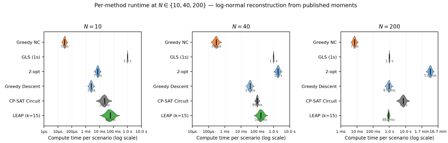
Figure 7: Per-method compute time at N \in \{10, 40, 200\} . Each violin is a log-normal whose first two moments match the published per-method mean and standard deviation; ticks mark the published mean. Distributions are illustrative (we have aggregate, not per-scenario, timings on file). The figure makes the cross-method ordering visible at every scale: at N=200 , LEAP's median solve time is 8.3 \times below the unpruned CP-SAT Circuit solver and slightly below the metaheuristics' fixed 1 s budget, while 2-opt with 50 restarts pushes past 5 minutes.
