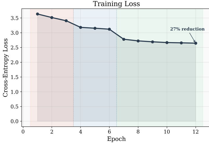
Figure 2: Cross-entropy loss over 12 epochs, coloured by curriculum stage.
