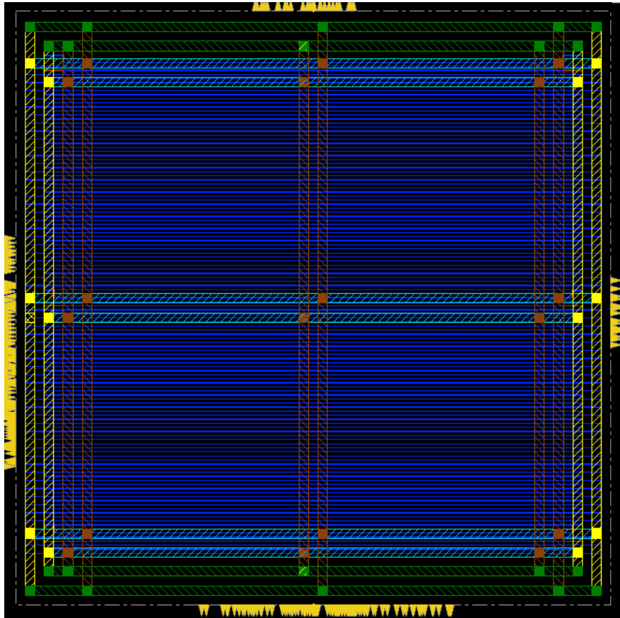
Figure 1.1: Power Distribution Network
