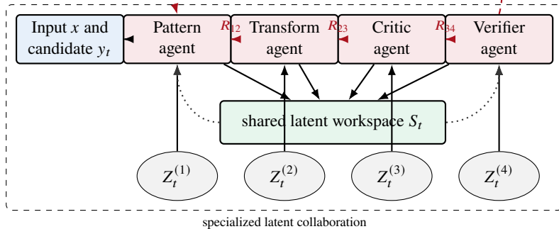
(b) Recursive Multi-Agent Tiny Recursive Model
