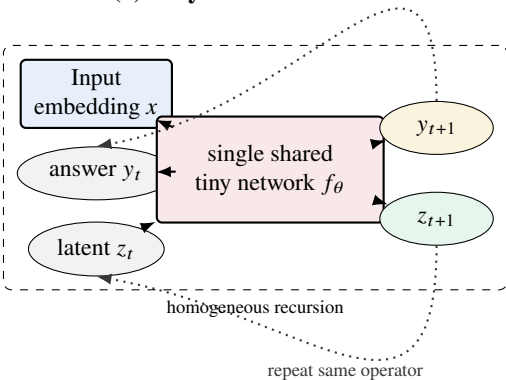
(a) Tiny Recursive Model
