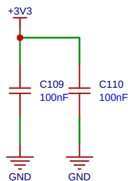
IMU 6DOF LSM6DSO32TR
