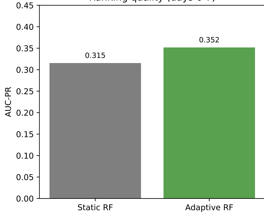
Ranking quality (days 6-7)
