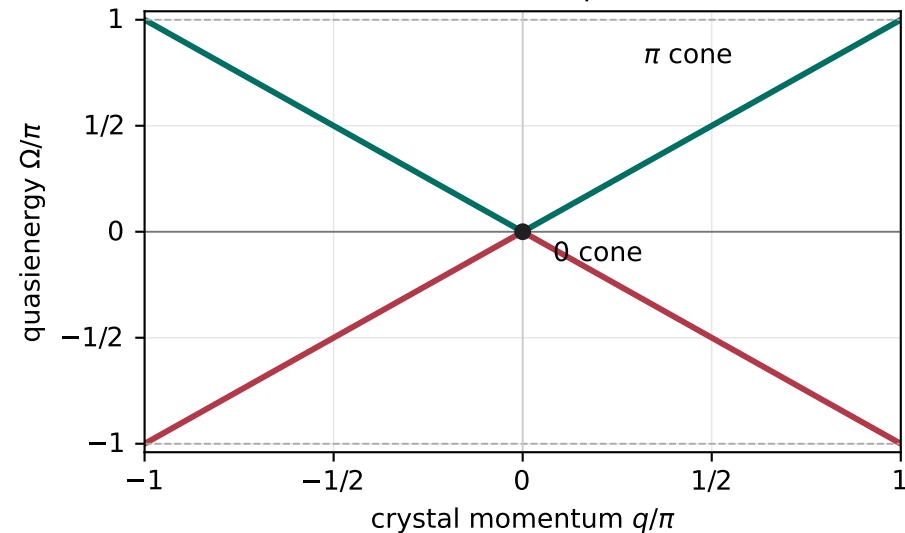
Massless: 0 and \pi cones
