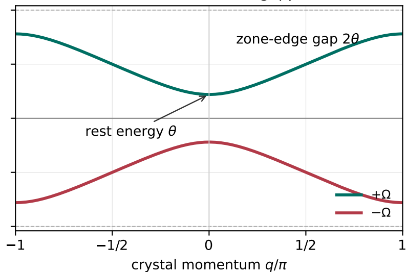
Massive: both cones gapped
