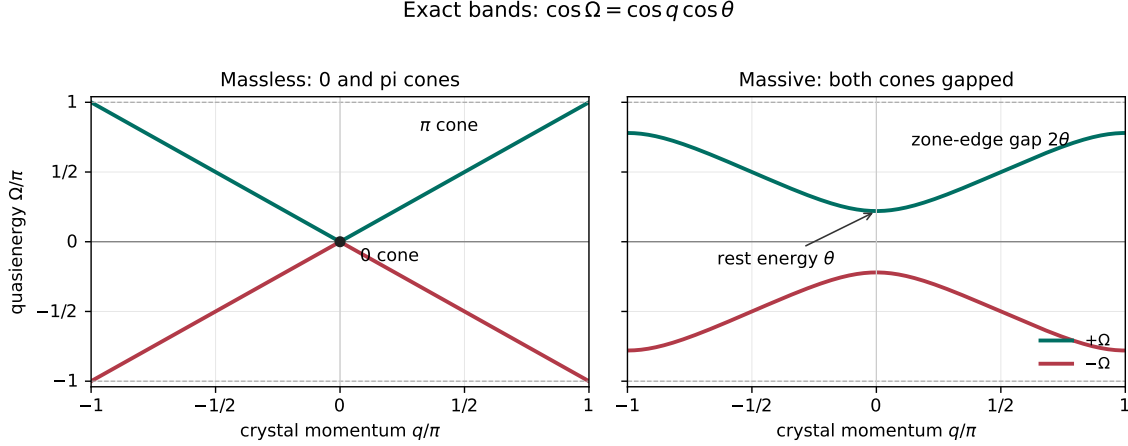
Figure 3: Exact quasienergy bands from \cos \Omega = \cos q \cos \theta . The left panel shows the massless cone at the origin and its Floquet partner at quasienergy \pi . A nonzero Plücker area opens both gaps (right). The curves evaluate the exact formula; they are not a fit or numerical simulation. Generated by Scripts/sim/plot_null_spinor_dirac_bands.py .
