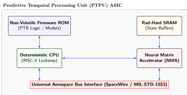
FIGURE 3 | Internal hardware architecture of the PTPU ASIC, highlighting the deterministic RISC-V lockstep CPU and the Neural Matrix Accelerator (NMA).
