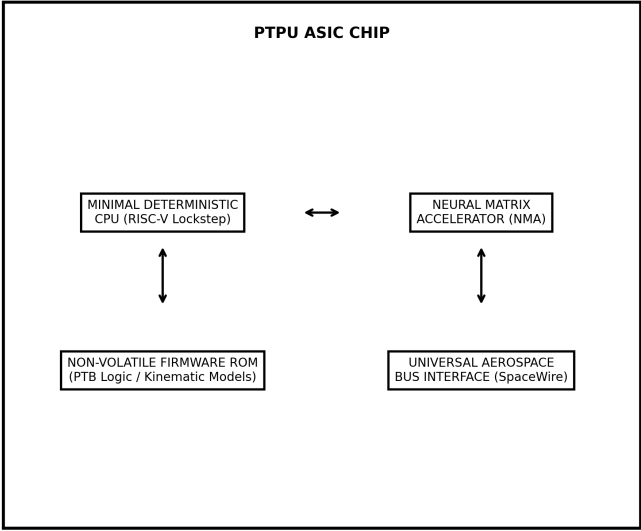
FIG. 2: PREDICTIVE TEMPORAL PROCESSING UNIT (PTPU) ARCHITECTURE
