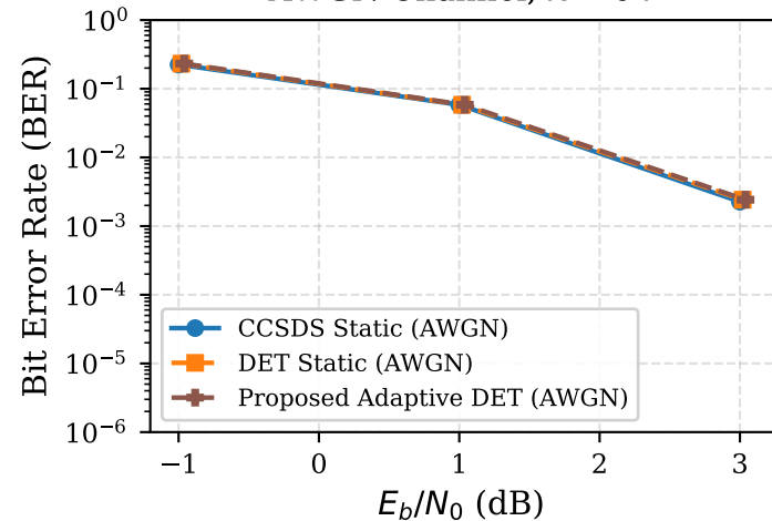
AWGN Channel, N = 64
