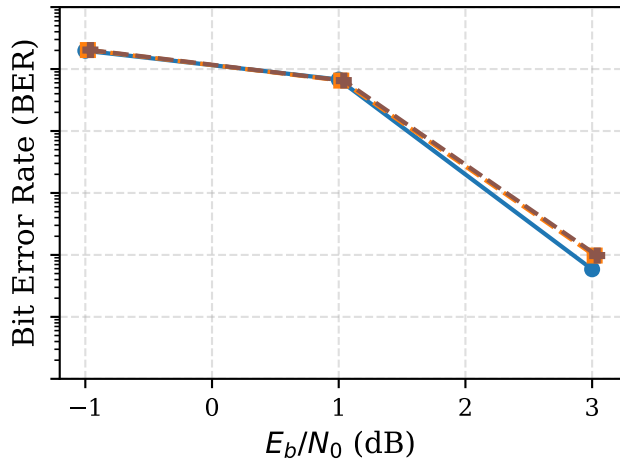
AWGN Channel, N = 256
