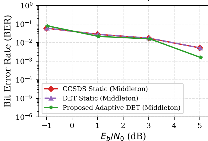
Middleton Class-A, N = 64
