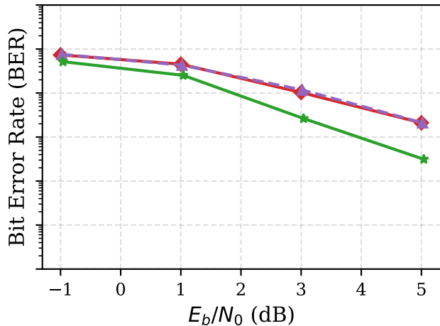
Middleton Class-A, N = 256
