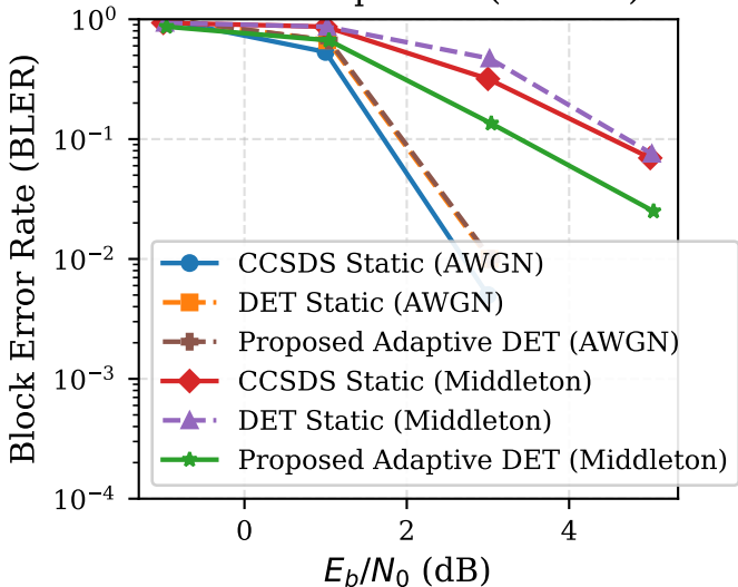
BLER Comparison ( N = 256 )
