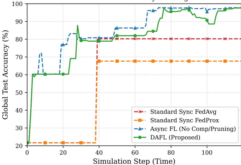
Global AI Model Accuracy Convergence
