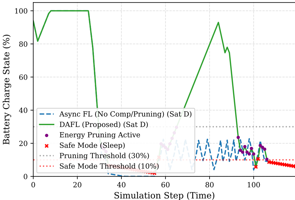
SmallSat Battery State-of-Charge Dynamics
