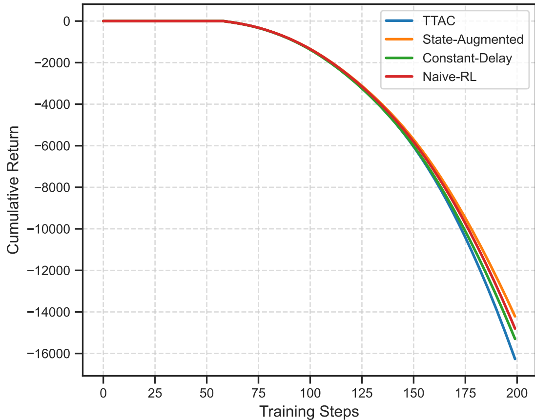
Sample Efficiency on Network Env
