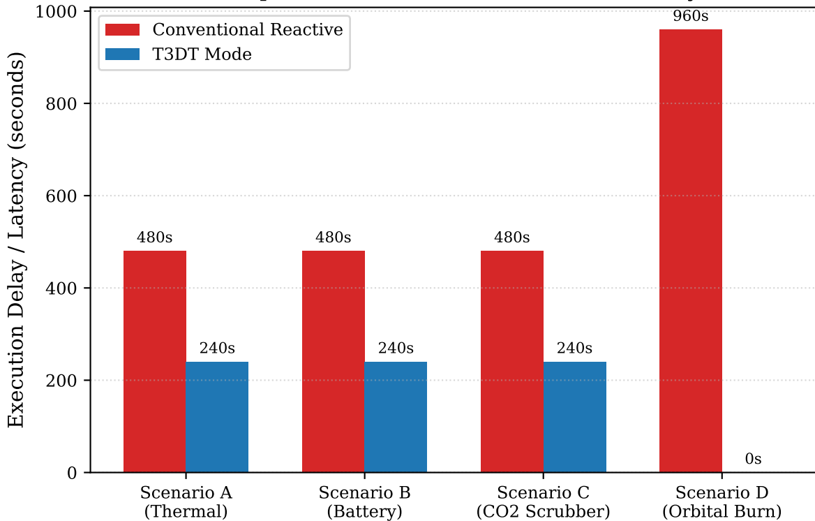
Comparison of Effective Command Latency
