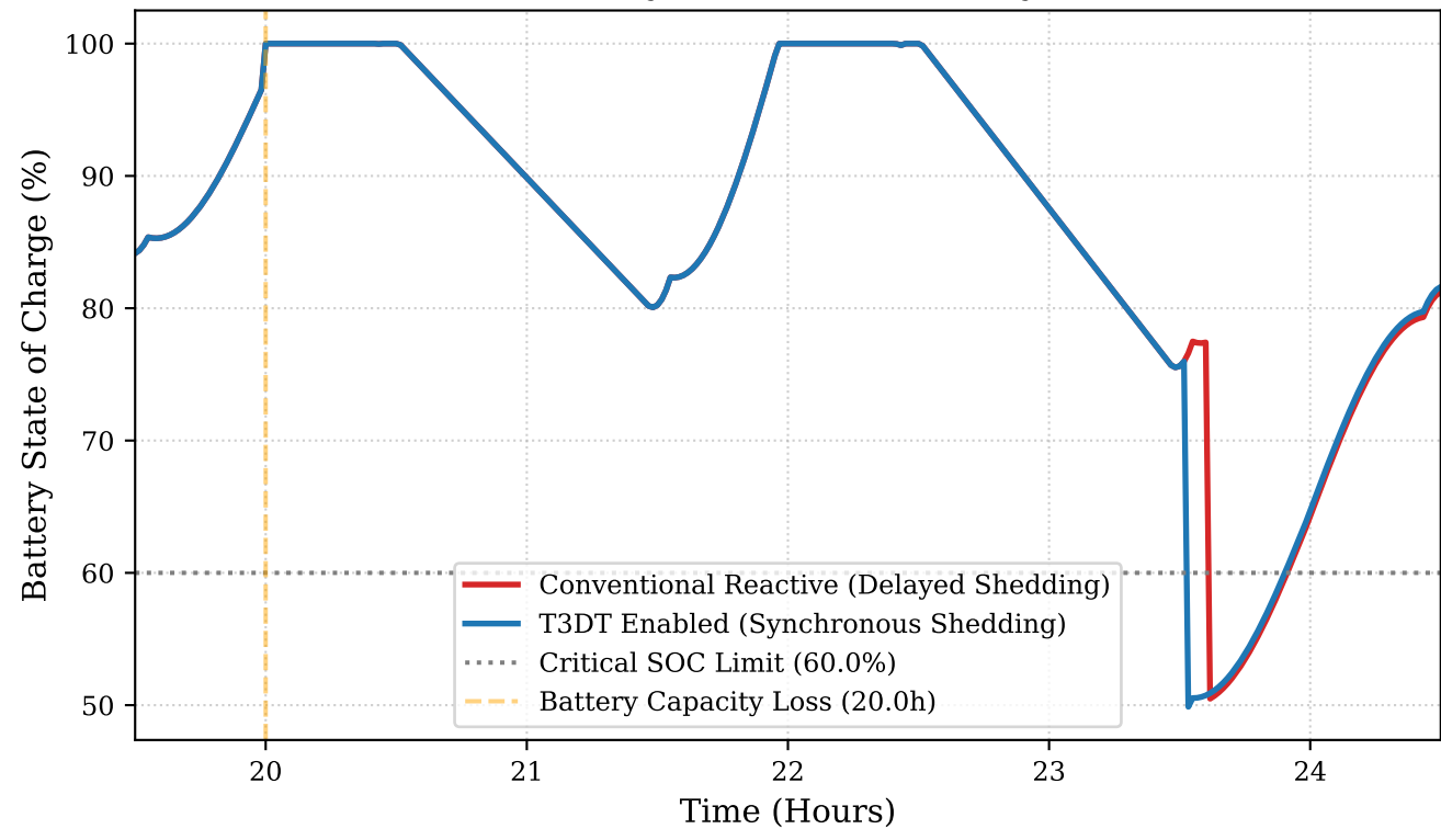
Electrical Power System (EPS) Recovery: Scenario B
