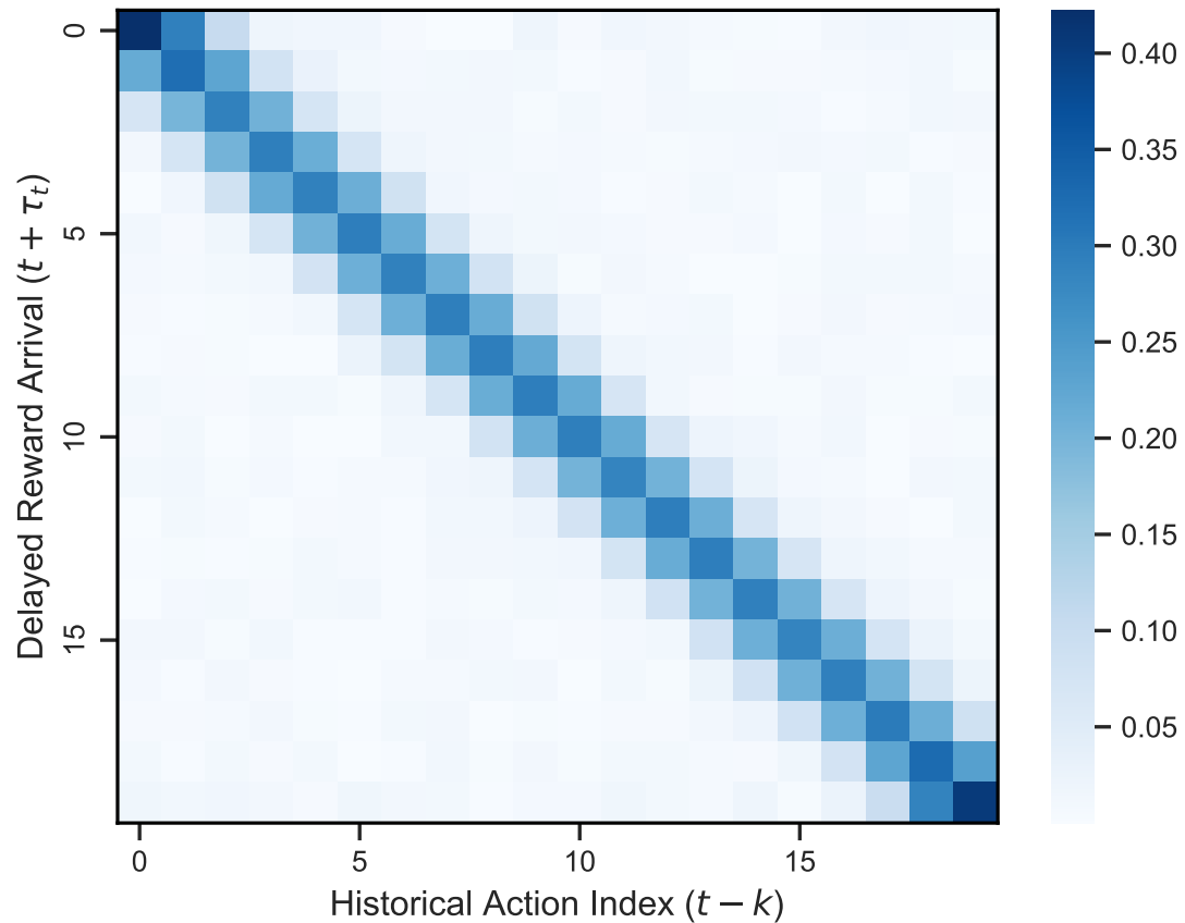
Retrospective Attention Matrix \mathcal{A}
