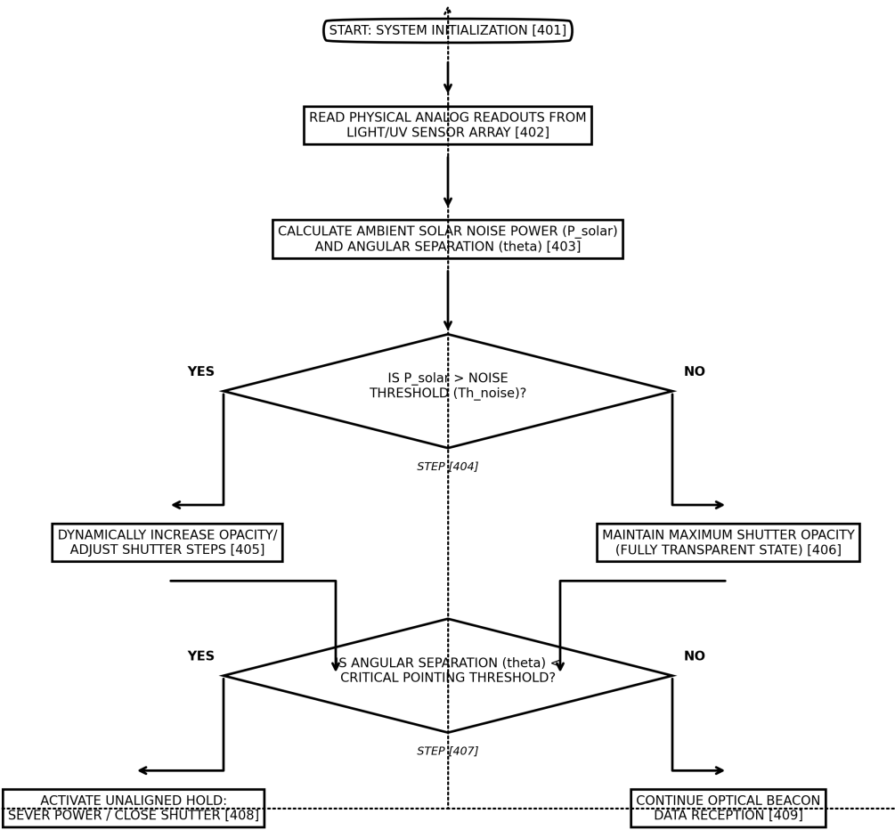
FIG. 4: REACTIVE SOLAR BLIND CONTROL METHODOLOGY FLOWCHART
