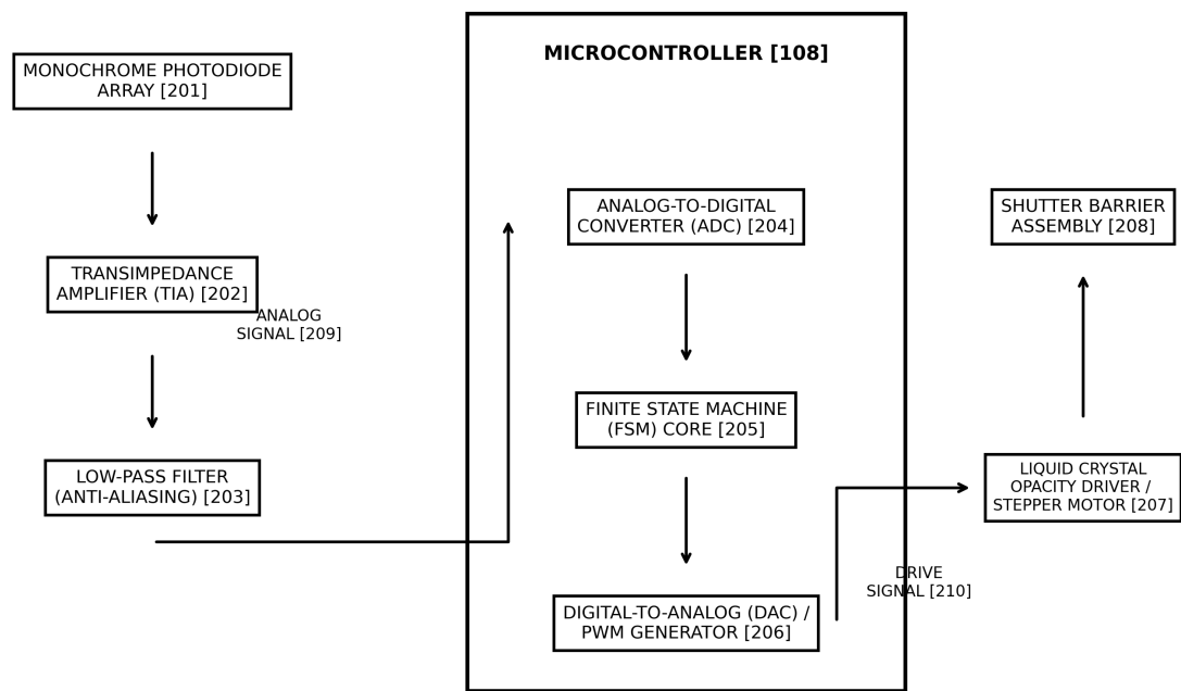
FIG. 2: SENSOR READOUT & SHUTTER ACTUATION ELECTRONIC SCHEMATIC
