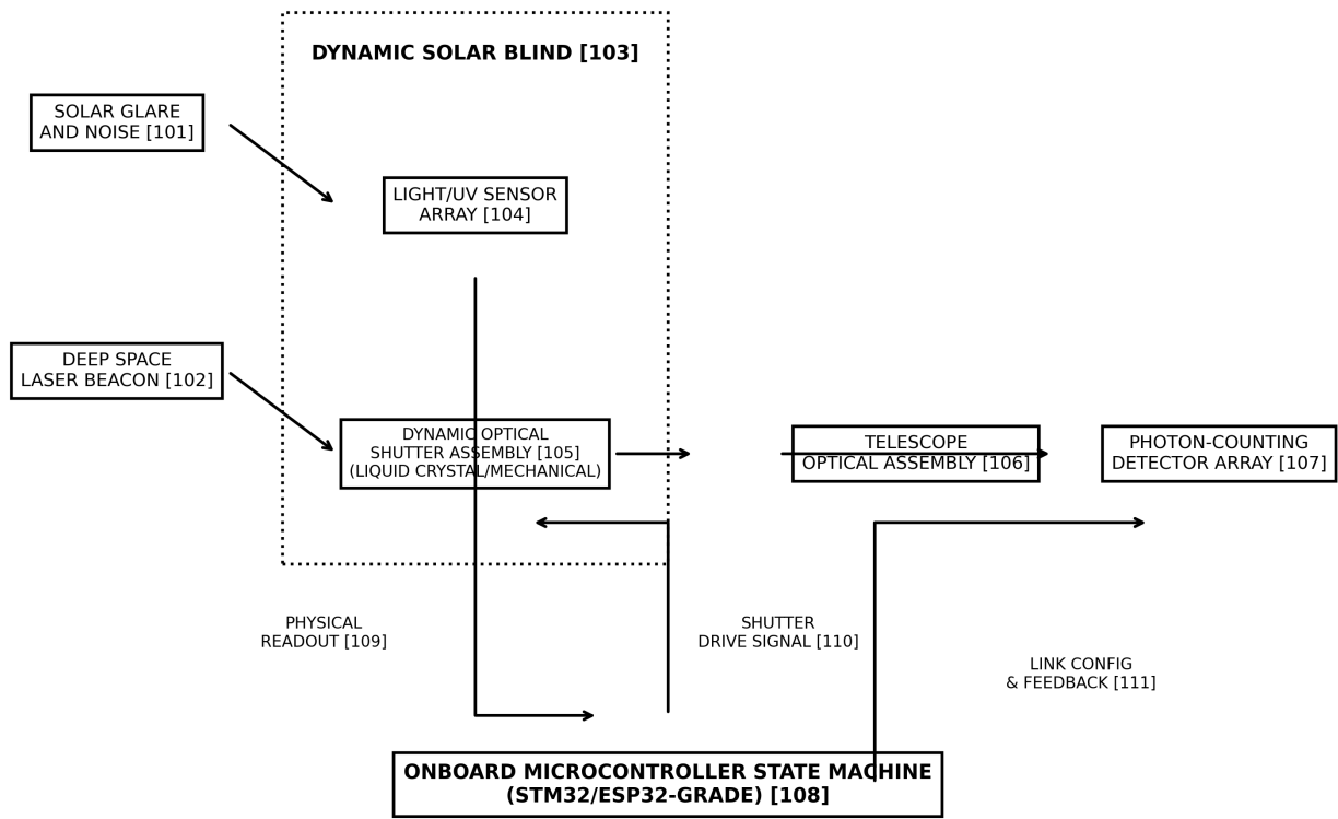
FIG. 1: DEEP SPACE OPTICAL TRANSCEIVER WITH DYNAMIC SOLAR BLIND ASSEMBLY
