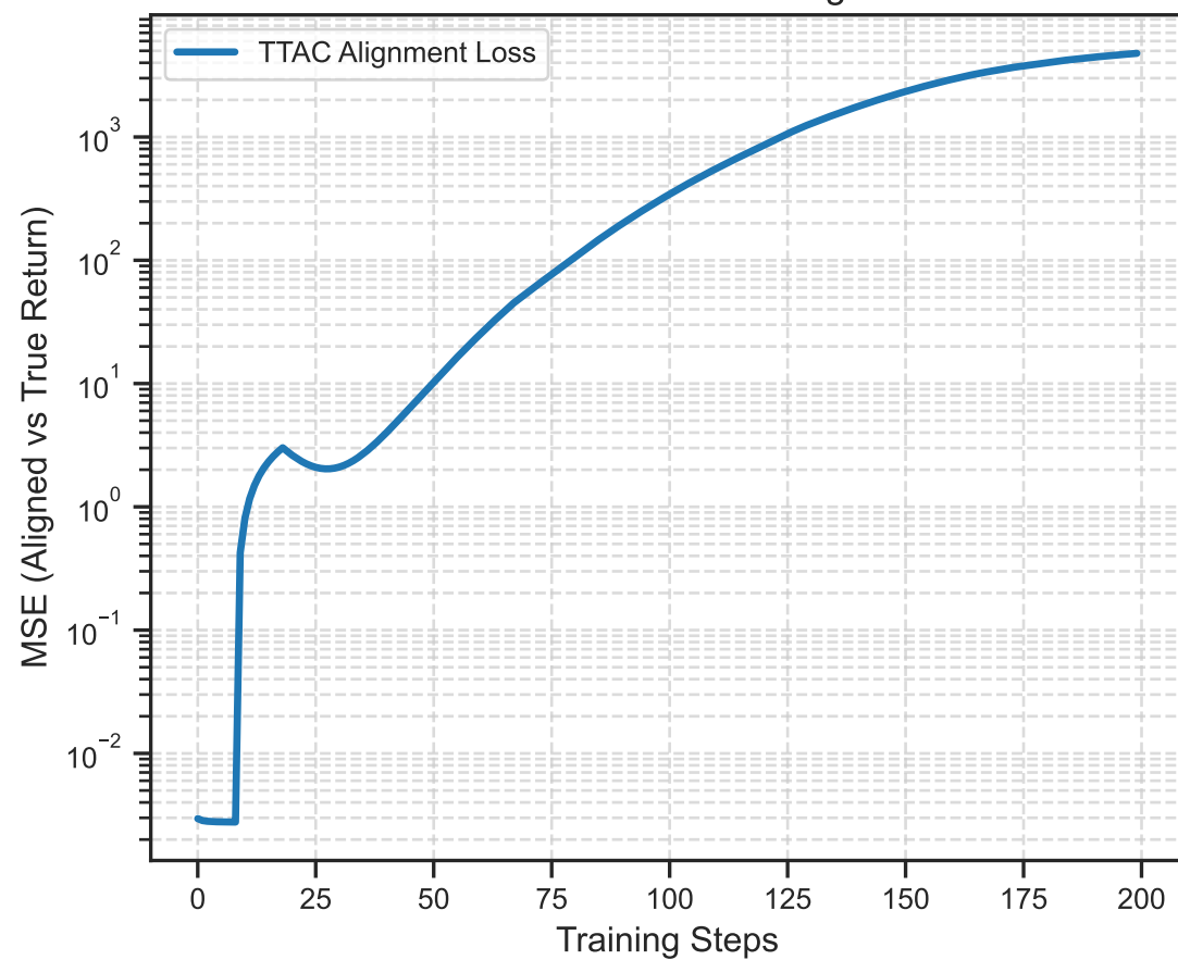
Pseudo-Reward Calibration / Alignment Loss
