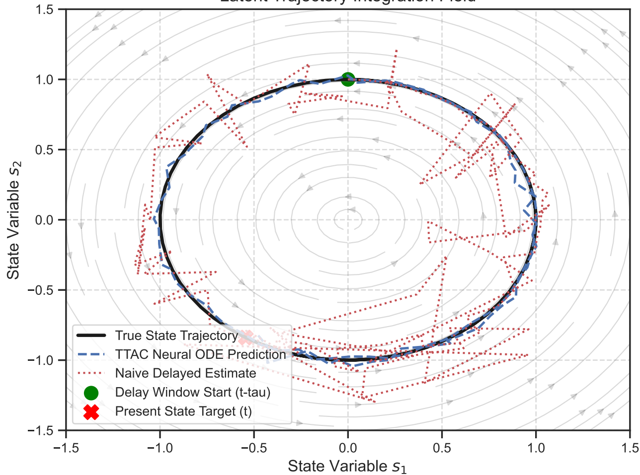
Latent Trajectory Integration Field
