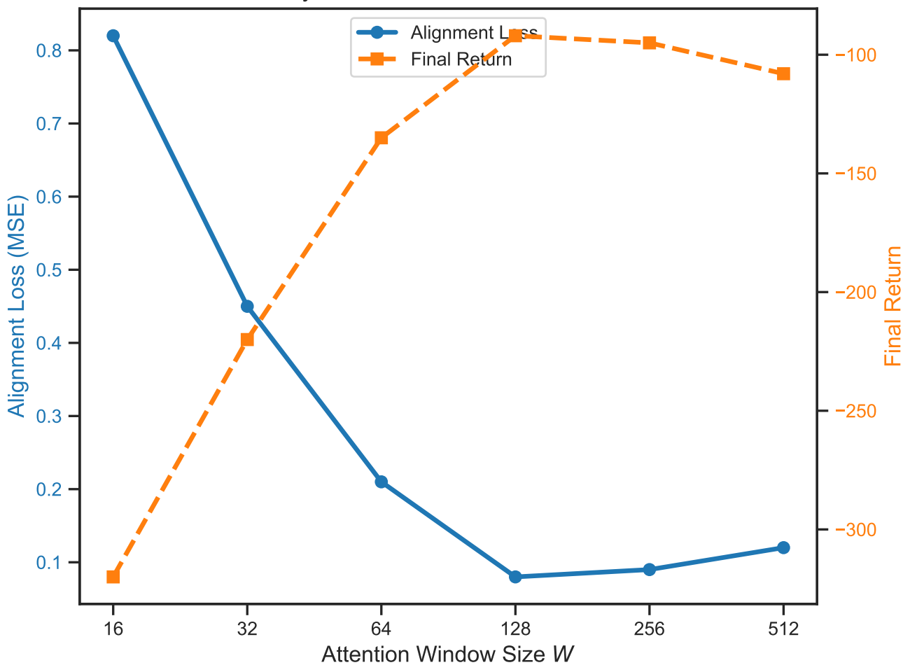
Sensitivity of Performance to Window Size W
