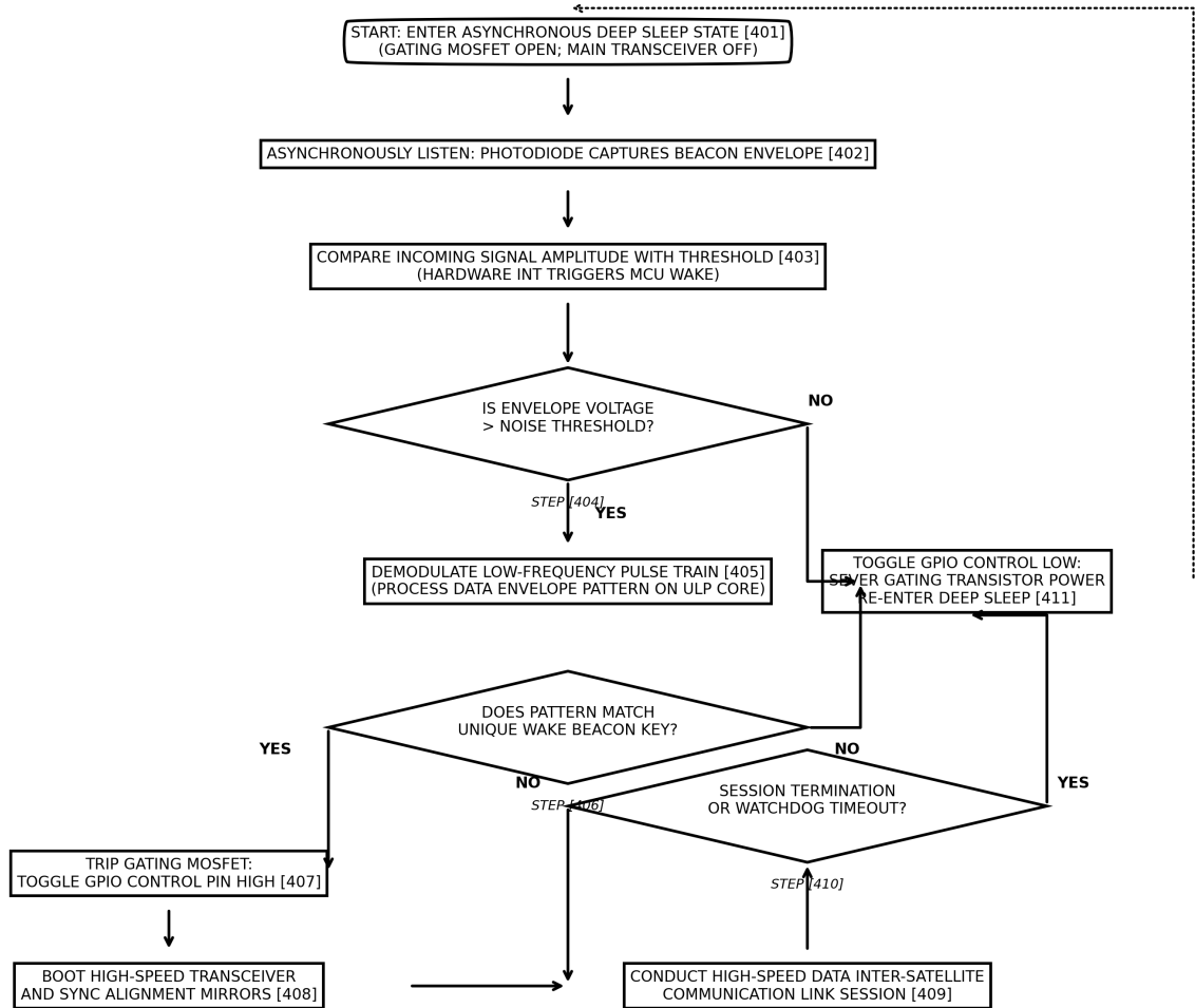
FIG. 4: LOW-POWER OPTICAL WAKE-ON-BEACON METHODOLOGY
