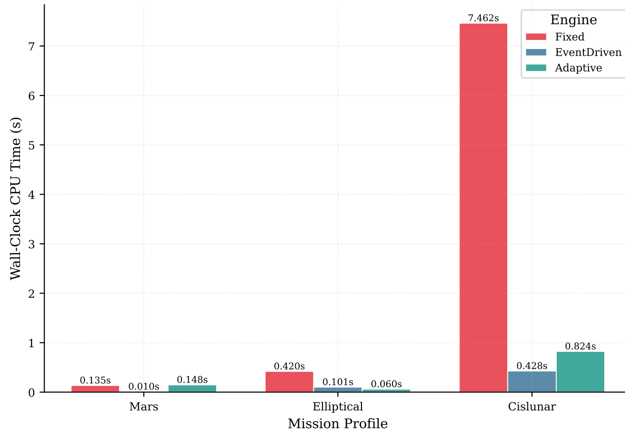
(a) CPU Execution Time by Engine and Profile
