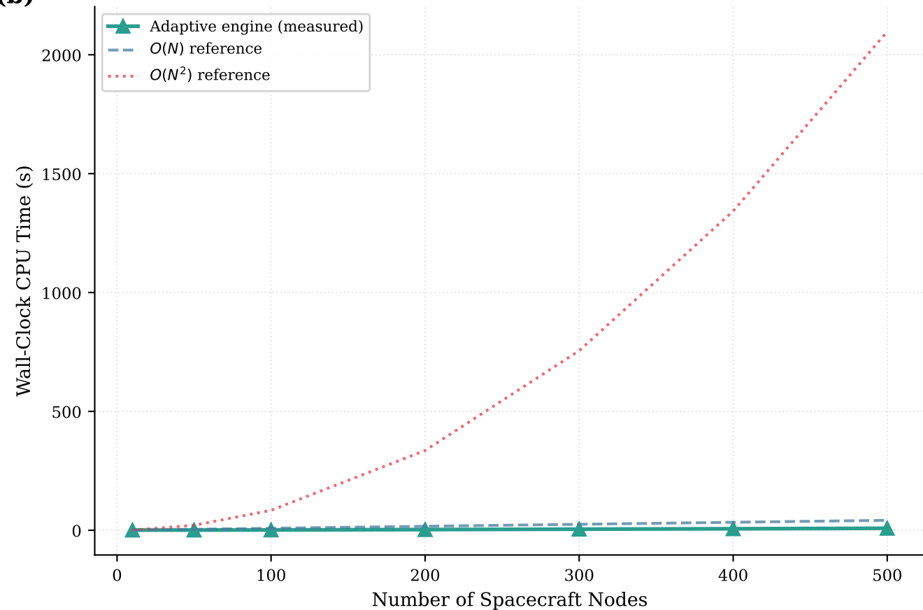
(b) Scalability: CPU Time vs. Node Count
