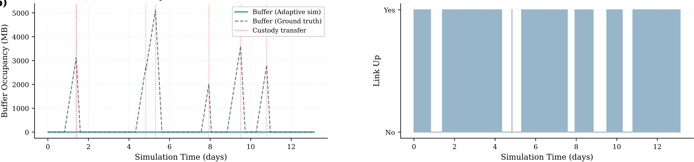
(b) DTN Buffer Dynamics — Cislunar NRHO
