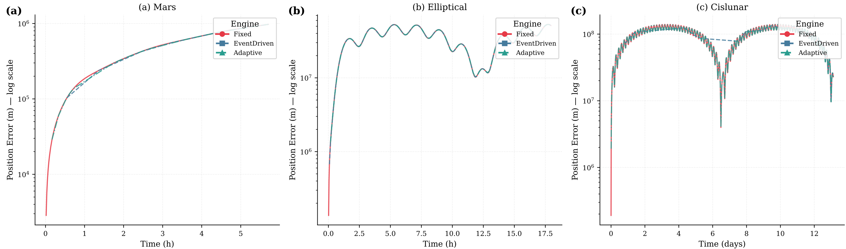
Figure 4 — Per-Step Position Error \varepsilon_{pos}(t) vs. Simulation Time
