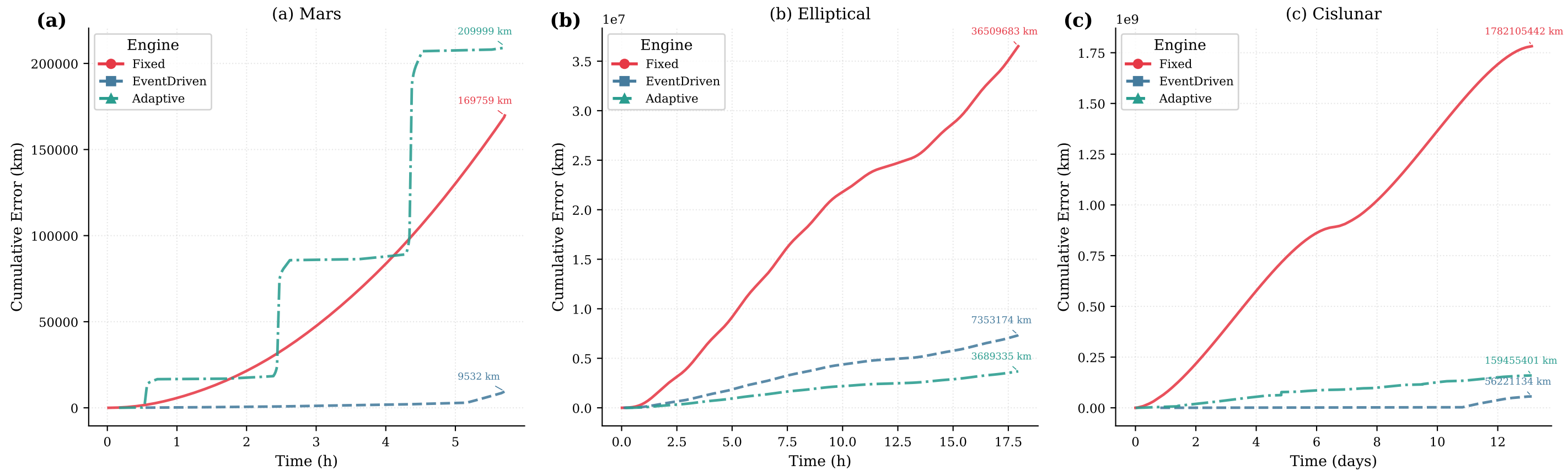
Figure 5 — Cumulative Integrated Position Error Growth
