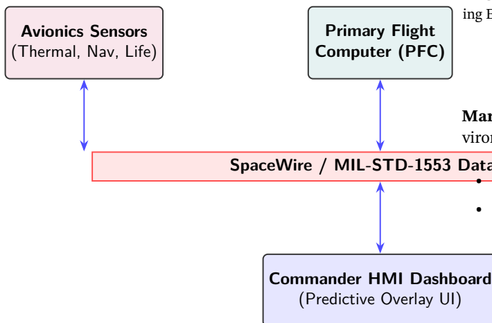
FIGURE 5 | Integration of the PTPU into the broader spacecraft avionics network via the SpaceWire / MIL-STD-1553 bus.
